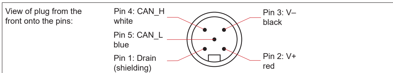
Fig. 27: Bus connection of DeviceNet with power supply
