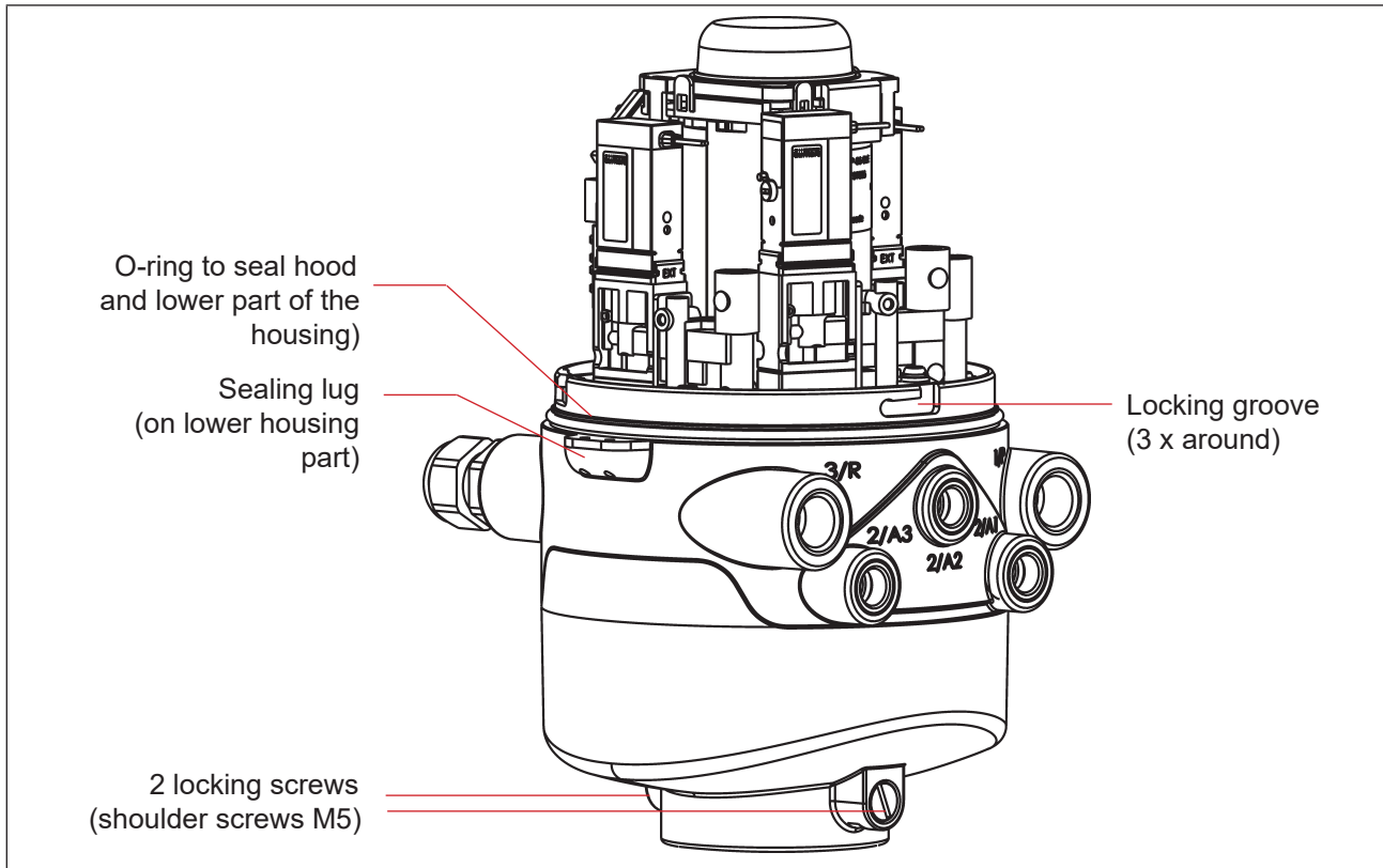
Fig. 16: Sealing and locking the housing
