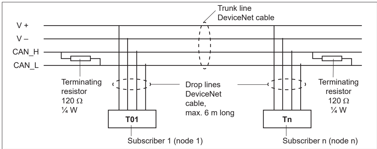
Fig. 29: Network topology
